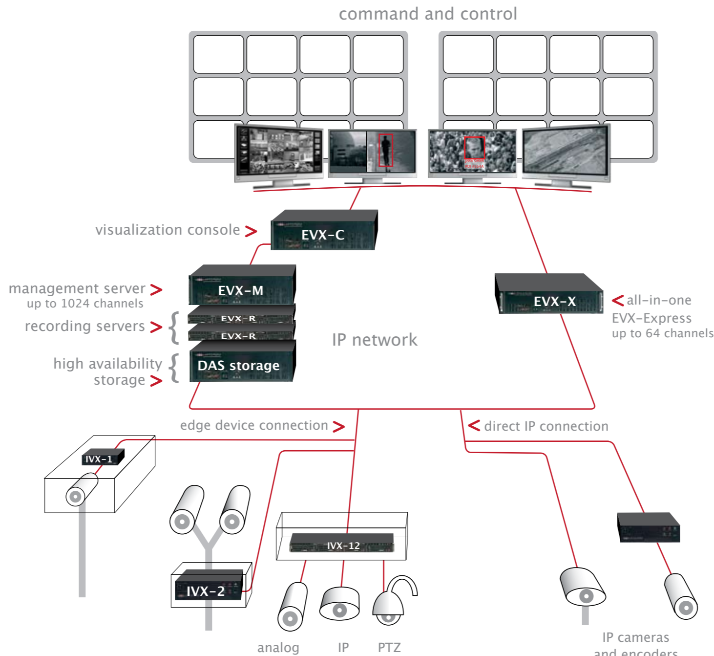
EVx range of enterprise video servers, IVx range of intelligent edge and central video devices
