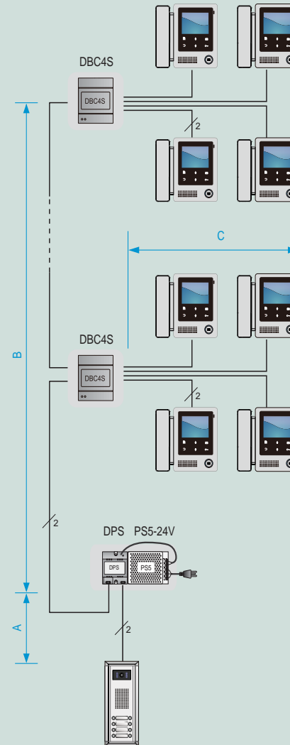
Connection Diagram
