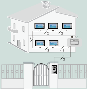
Extending Monitors(up to 16)
