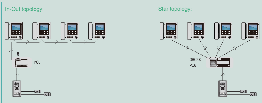
Extending Monitors(up to 16)
