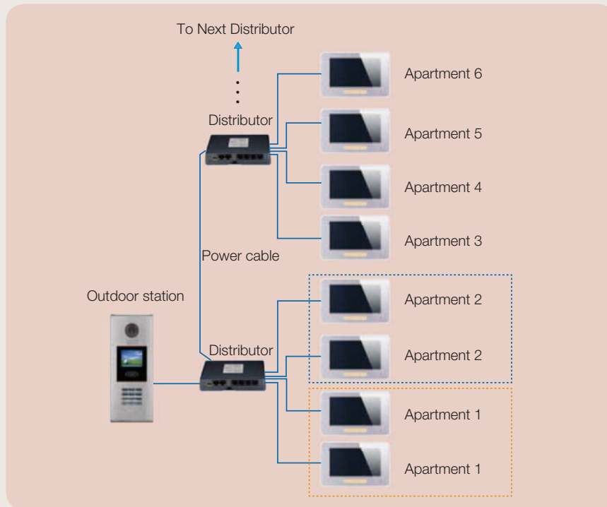
Cable limitation and power distribution table
