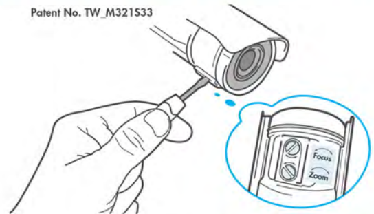
Accommodate view length from 3 to 10.5 mm @ F1.4
